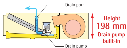
Ceiling concealed
