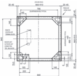
Upper View
