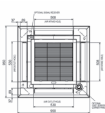
Lower View
