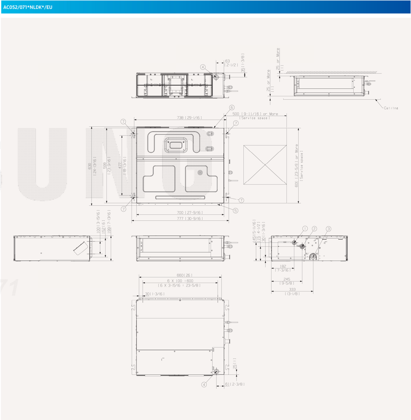
LSP Duct (Duct S)
